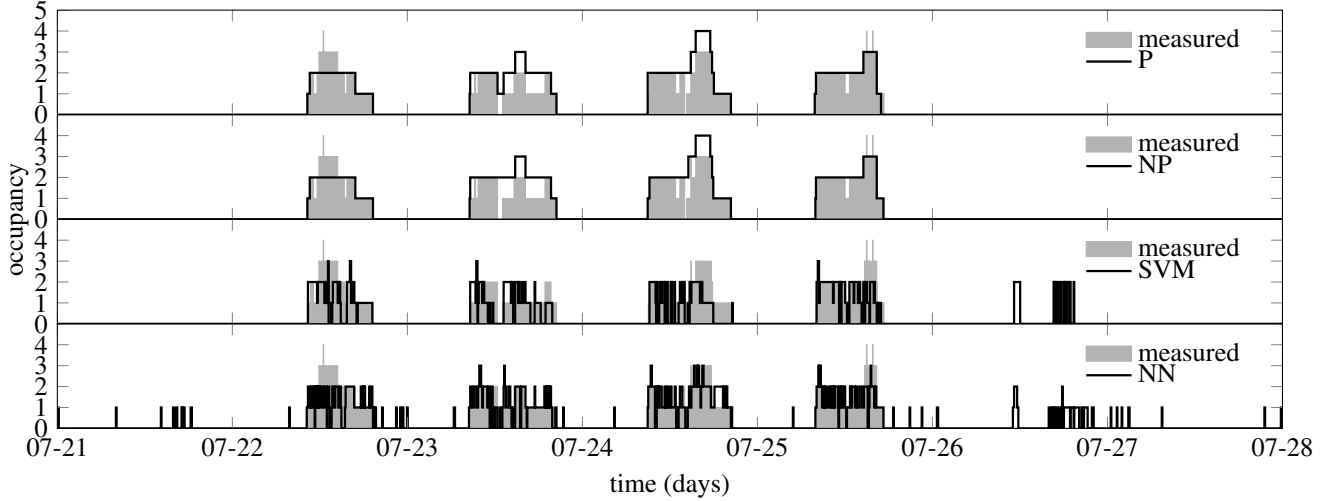
Figure 3. Realizations of the estimation processes for the test set considered in our experiments.
